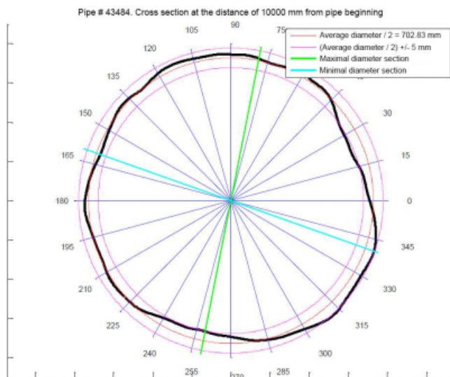
Figure 6.2. Pipe profile (shown in the enlarged scale near the pipe surface)
